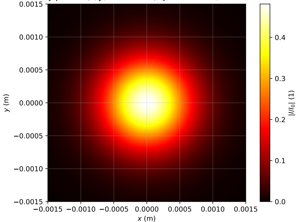
Intensity profile I(x, y, z = 3.423m)/I_0 , Pin=0.5Pcr, artificial time
